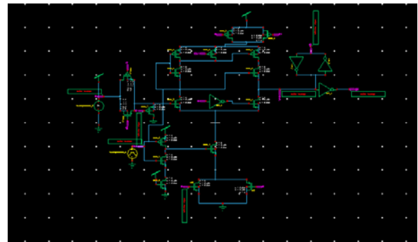
Fig.4 Edge Trigger Design With Sleepy Stack Technique
